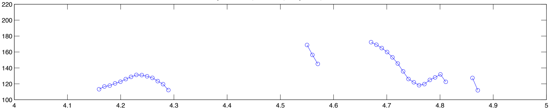
Voicebox pitch tracker; smoothed, interpolated, outliers removed.
